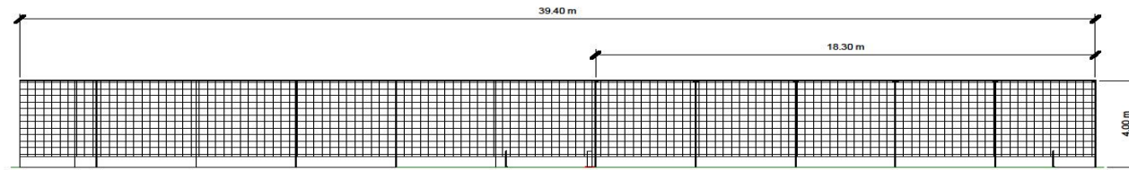
Cage Elevations Scale 1:100
